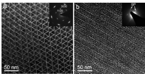
Figure 2. TEM images of the edge-to-edge (a) and face-to-face (b) superlattices (SP) of LaF 3 nanoplates. Insets are the SAED patterns.
